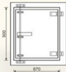
Porta laterale supplementare obbligatoria per kit IR Side supplementary door is obligatory for IR kit - Porte laterale supplémentaire obligatoire pour IR kit Puerta lateral suplementaria obligatoria para el kit
