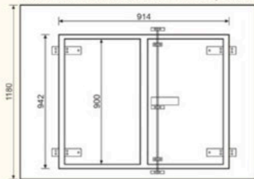
PORTA LATERALE SUPPLEMENTARE - SUPPLEMENTARY SIDE DOOR PORTE LATERALE SUPPLÉMENTAIRE - PUERTA LATERAL SUPLEMENTARIA
